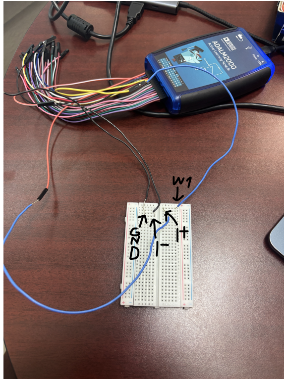
Figure 1. Labeled physical wiring photograph: W1 → 1+ and GND → 1-.
